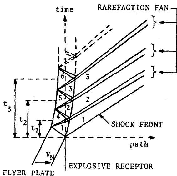
Fig 10 Principle of Generation of Rectangular Pressure Pulses
